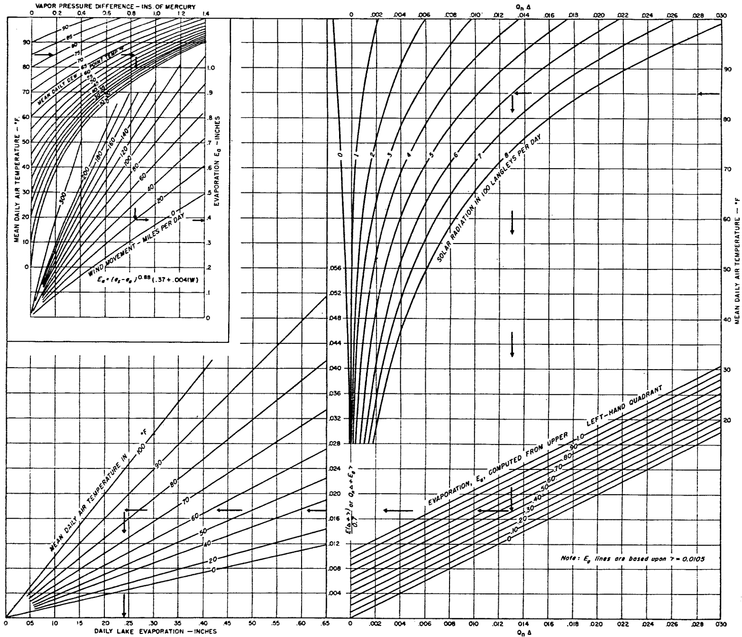
FIGURE 6.—Graphical presentation of equation (10).
