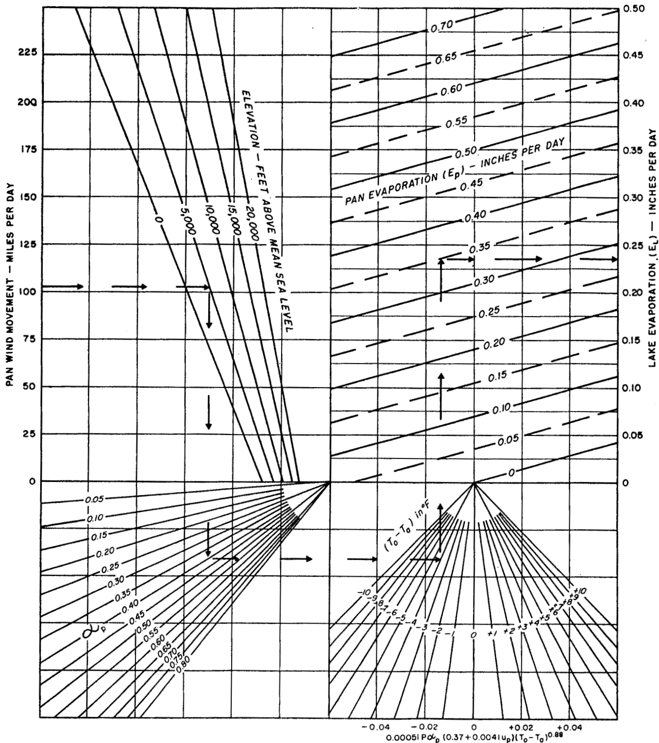
FIGURE 7.—Graphical presentation of equation (14).
