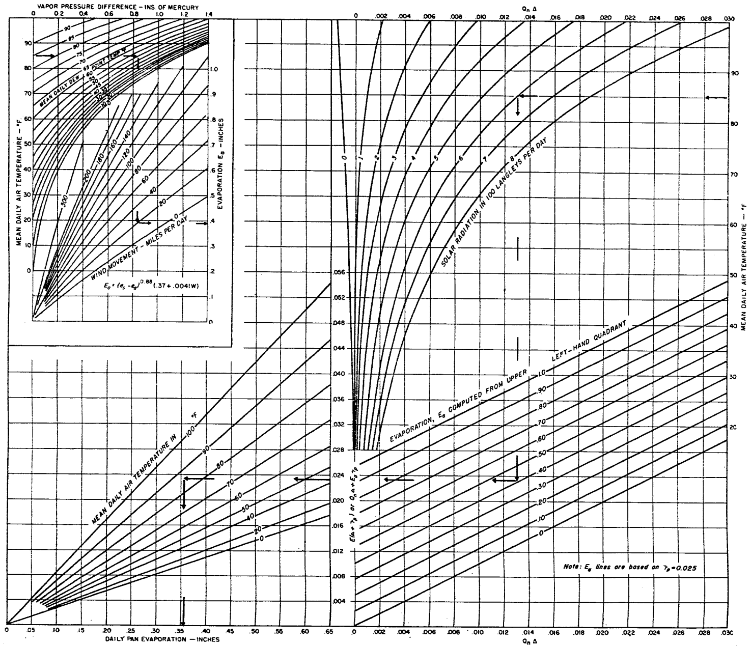
FIGURE 2.—Revised relation for Class A pan.
