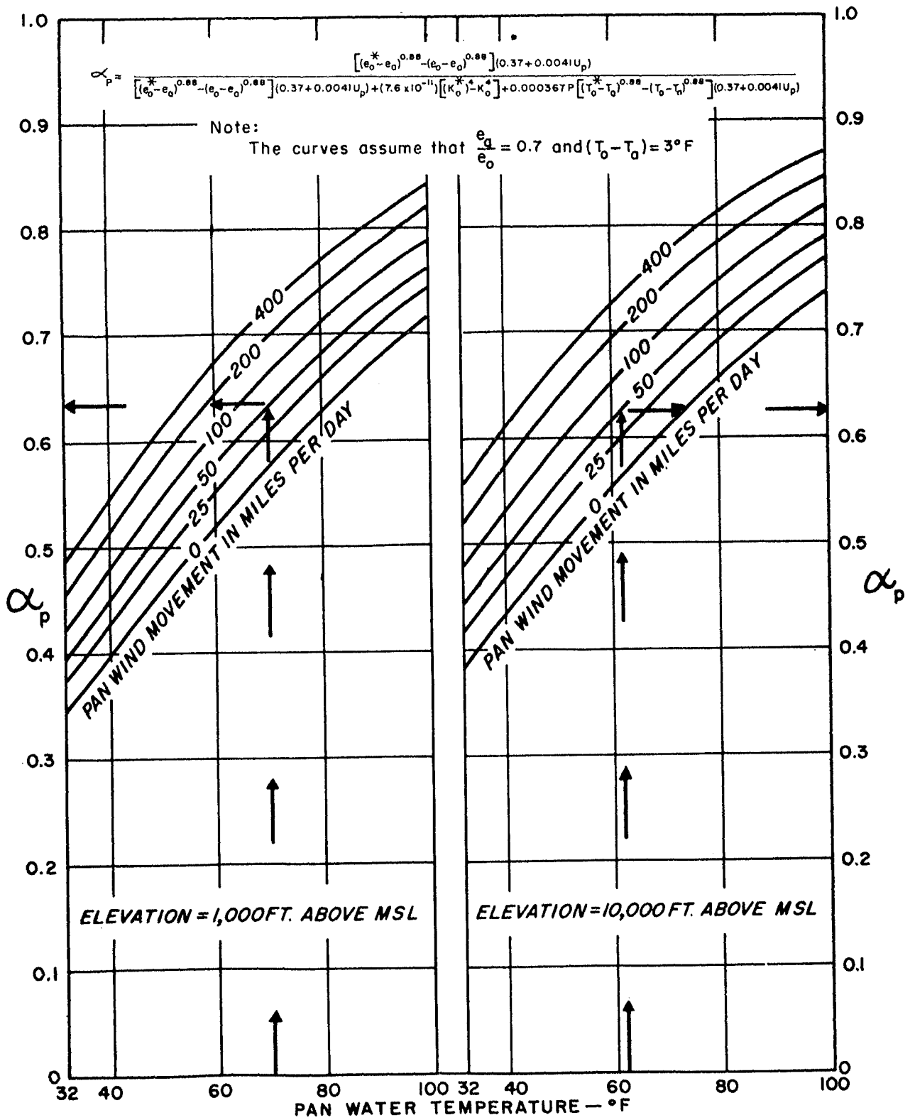
FIGURE 5.—Proportion of advected energy (into a Class A pan) utilized for evaporation.
