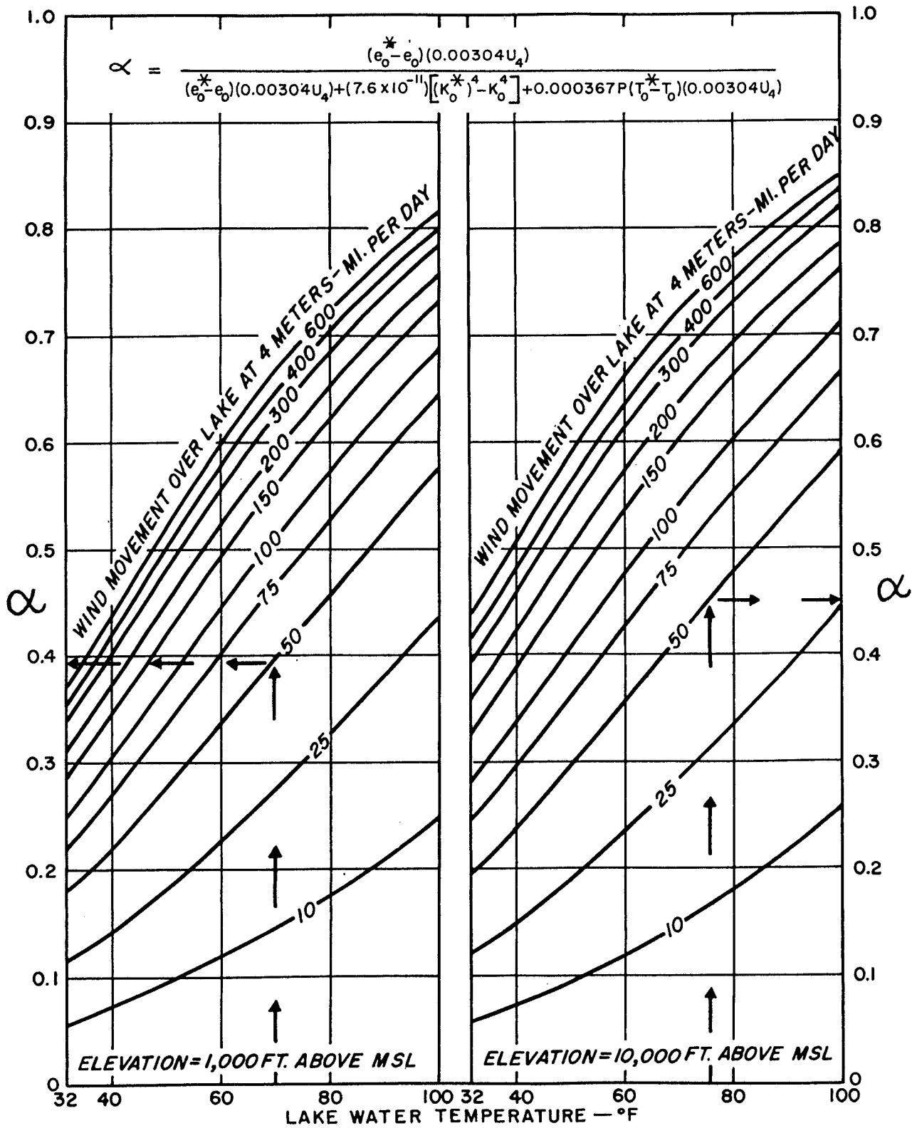
FIGURE 4.—Proportion of advected energy (into a lake) utilized for evaporation.
