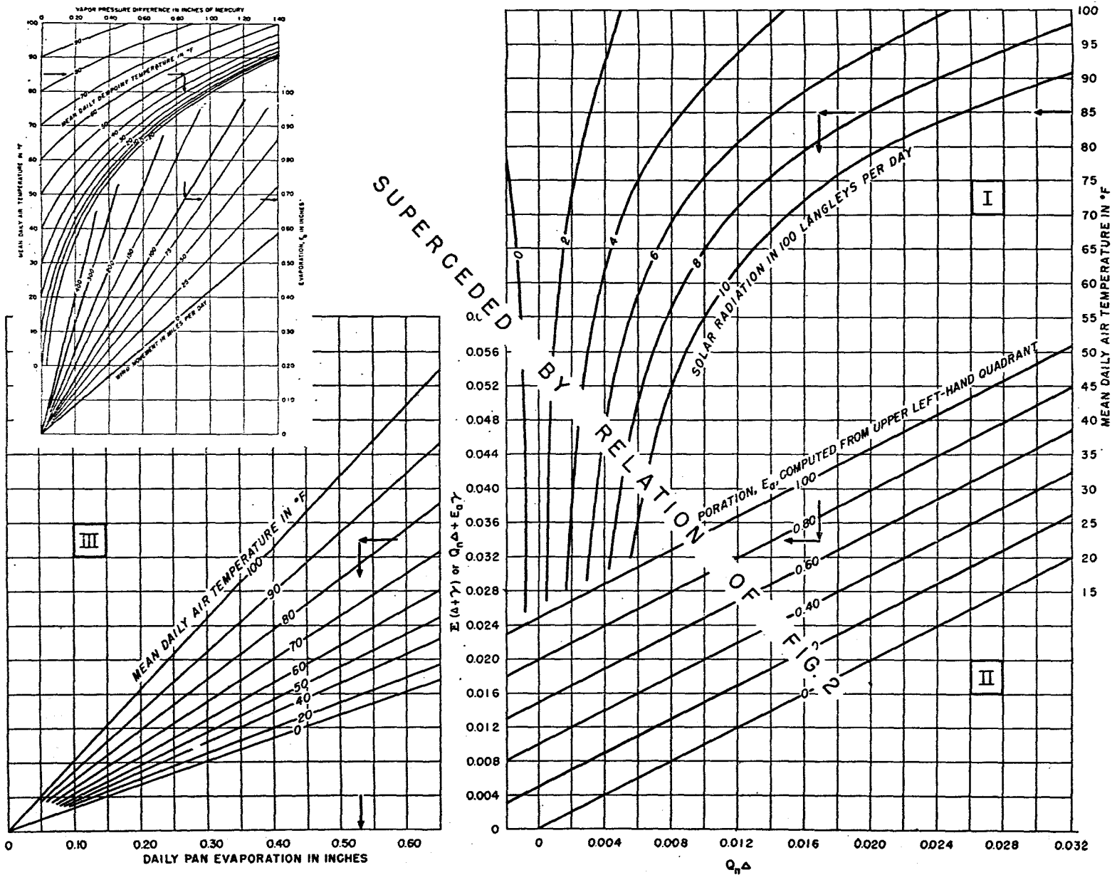
FIGURE 1.—Relation for Class A pan, based only on observations from Lake Hefner South Station.
