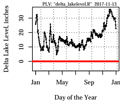
Delta Lake Level and LRB Year = 2004
