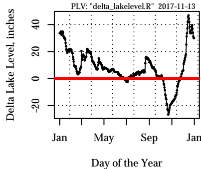
Delta Lake Level and LRB Year = 2007
