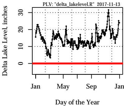
Delta Lake Level and LRB Year = 2003
