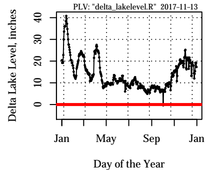
Delta Lake Level and LRB Year = 2005
