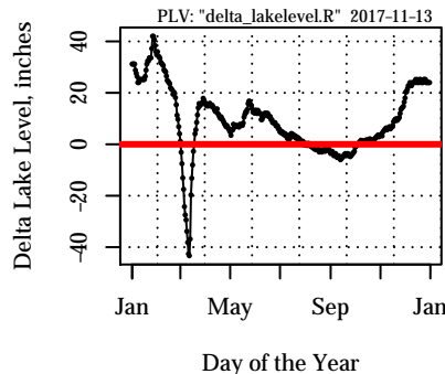
Delta Lake Level and LRB Year = 2010
