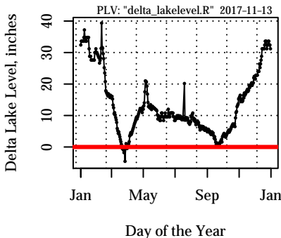
Delta Lake Level and LRB Year = 2009
