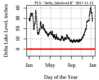
Delta Lake Level and LRB Year = 2008
