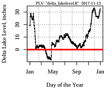
Delta Lake Level and LRB Year = 2006
