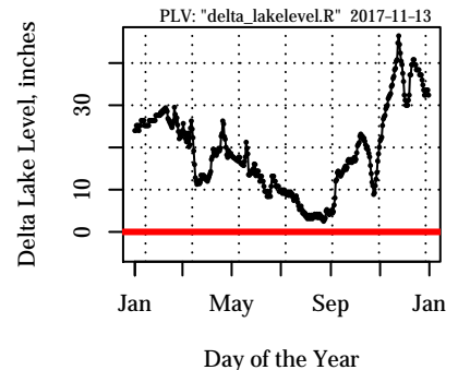
Delta Lake Level and LRB Year = 2011
